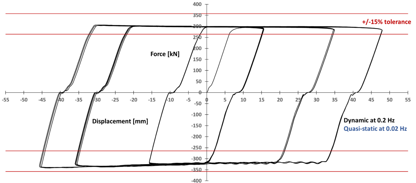
High-consistent dynamic performance of Tectonus DMAX brace with a tolerance lower than +/-15% (as per ASCE07-16)
